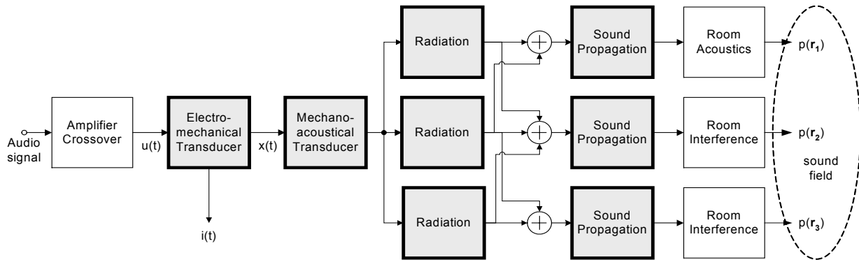
Fig. 1. Signal flow in a sound reproduction system
