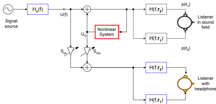
Fig. 2: Auralization technique illustrated by a signal flow chart between signal source and listener
