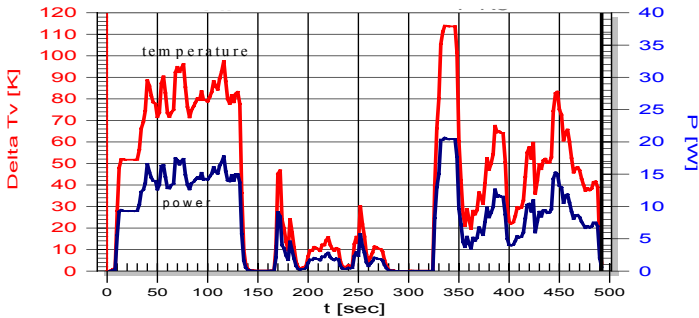
Fig. 4: Input power and voice coil temperature during the reproduction of three stimuli
