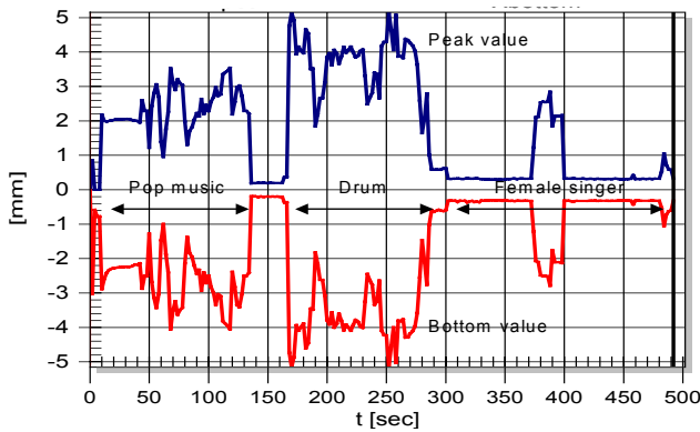
Fig. 3: Voice coil displacement during the reproduction of three stimuli
