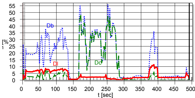
Fig. 5: Ratio of distortion components D_b , D_c , D_l generated by force factor Bl(x) , compliance C(x) and inductance L(x) , respectively, during the reproduction of three stimuli
