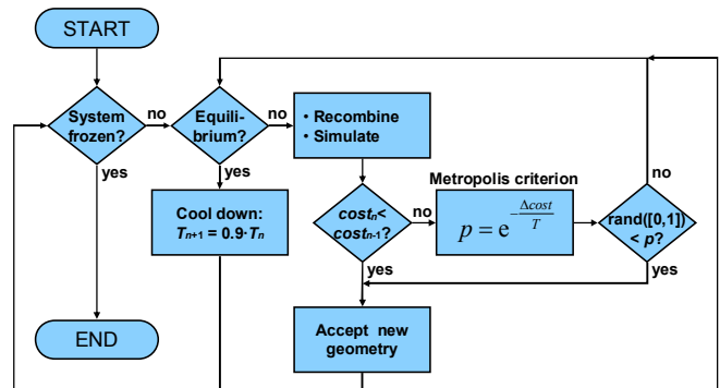
Figure 2: Inhomogeneous simulated annealing algorithm
