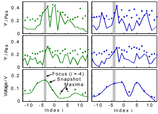
Figure 6: Spatial focusing – best (left) and coincidental system (right) – single channel (top) and four channel simulation (middle), measured voltages of the experiment (bottom)
