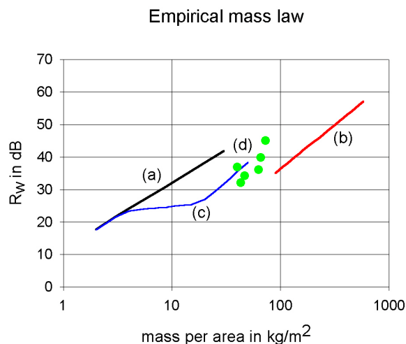
Figure 3: mass law for single leaf walls :
