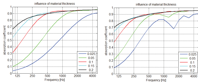
Figure 5: Calculated sound absorption of glasswool with air flow resistivity 12,9 kPa.s.m -2 and thickness of the material. Left: with hard backing, right: with an air gap of 100 mm.
