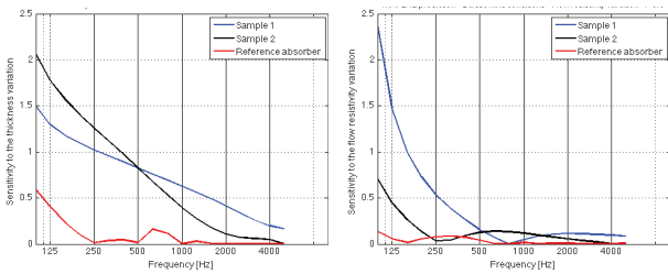
Figure 3: Calculated sensitivity of the sound absorption for variation of an input parameter, glasswool air flow resistivity 12,9 \text{ Pa.s.m}^{-2} with three thicknesses. Left: for thickness variation, right: for air flow resistivity variation.
