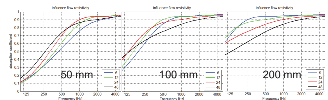
Figure 4: Calculated sound absorption for different air flow resistivity (in \text{kPa.s.m}^{-2} ) and thickness of the material.
