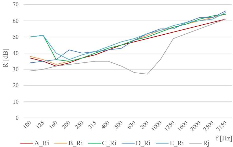
Figure 5 – Input values of the sound reduction index R_i of the different configurations of façade and the sound reduction index R_j of the lateral elements.
