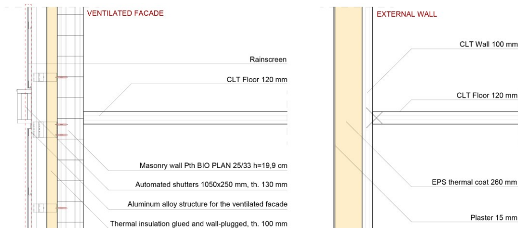
Figure 2 – Construction details: the ventilated façade-floor (left) and external wall-floor junction (right).
