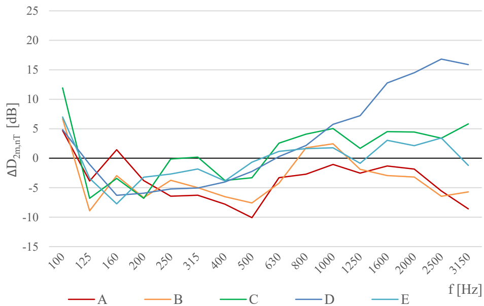
Figure 8 – Difference between measured and calculated values of the standardized sound level difference of the façade considering the model “ISO 12354_Var. 3”.
