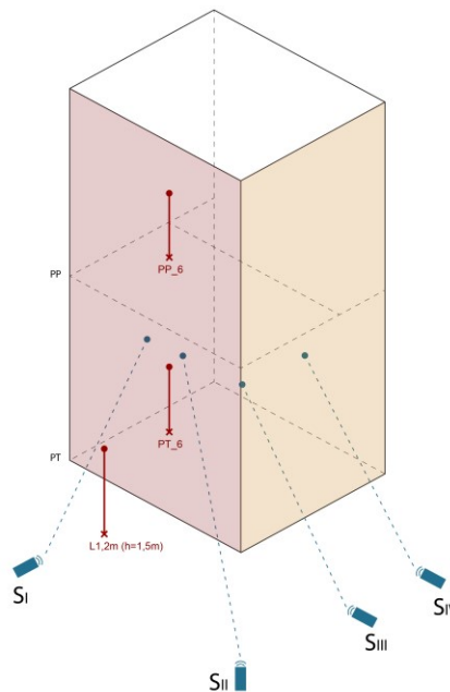
Figure 3 – Scheme of the measurement setup used with indication of the position S_I , S_{II} , S_{III} , S_{IV} sources.
