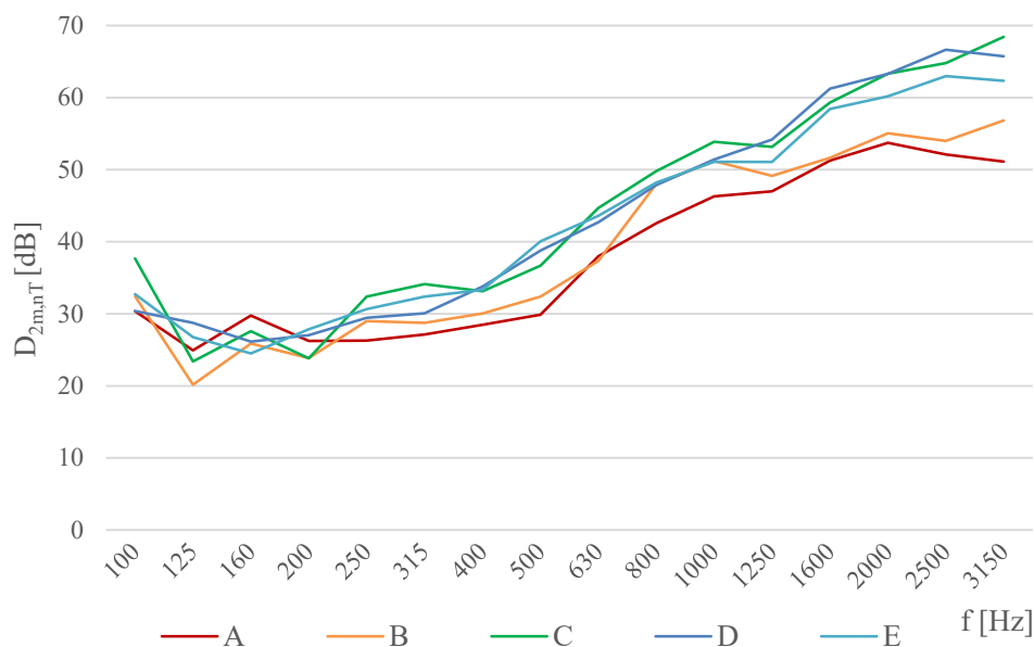
Figure 4 – Standardized sound level difference of façade measured on site in one-third octave bands.
