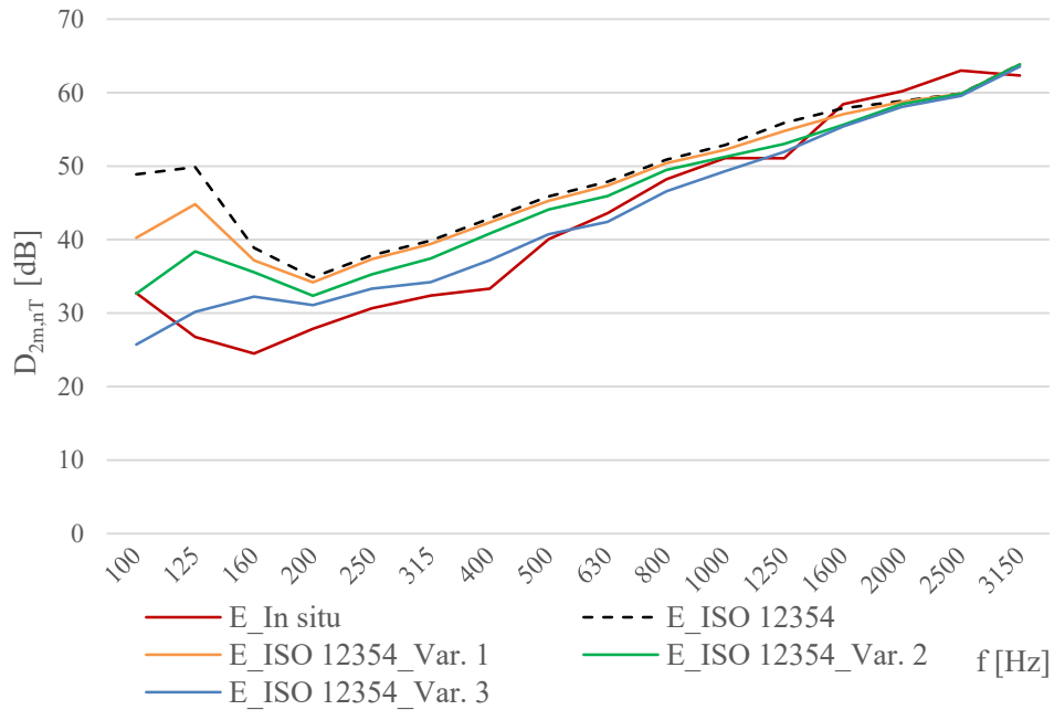
Figure 7 – Difference between measured and calculated values of the standardized sound level difference of E configuration in relation to different variables.
