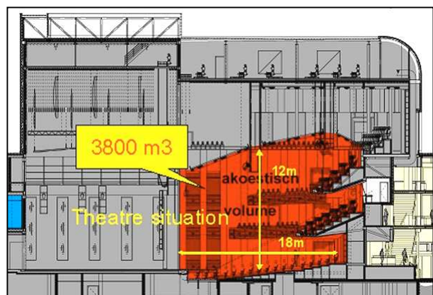
Figure 9: Cross-section of theatre De Spiegel in Zwolle (2006, V=3,800-11,000 m 3 ) in theatre mode. The red area indicates the acoustical room volume (V=3,800 m 3 ).
