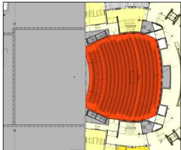
Figure 8: Plan (ground floor) of theatre De Spiegel (2006, V=3,800-11,000 m 3 ) in theatre mode. The red area indicates the acoustical room volume.
