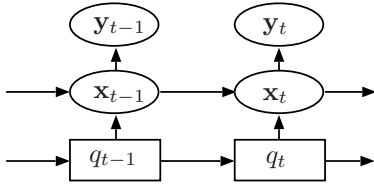
Figure 1: Bayesian network considering temporal correlation between features.
