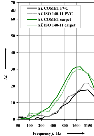
Figure 7: Impact noise reduction \Delta L [dB], timber: COMET vs. ISO procedure
