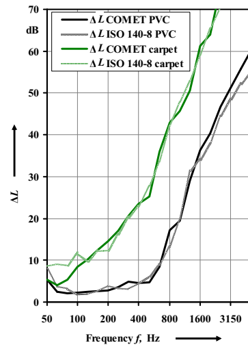
Figure 4: Impact noise reduction \Delta L [dB], concrete: COMET vs. ISO procedure
