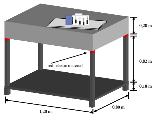
Figure 2: Construction of COMET, concrete floor
