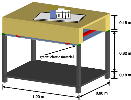
Figure 3: Construction of COMET, timber floor
