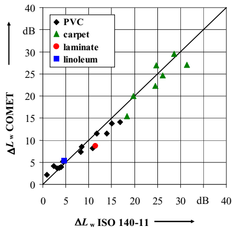
Figure 9: Deviation of \Delta L_w [dB], timber: COMET vs. ISO procedure
