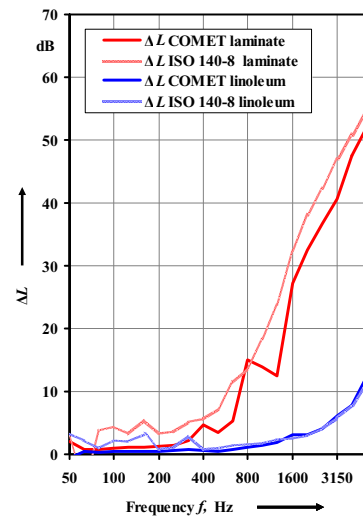
Figure 5: Impact noise reduction \Delta L [dB], concrete: COMET vs. ISO procedure
