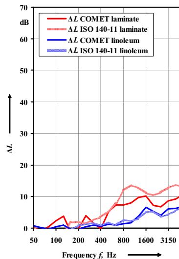
Figure 8: Impact noise reduction \Delta L [dB], timber: COMET vs. ISO procedure
