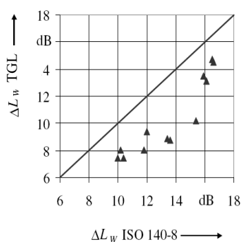
Figure 1: Difference of \Delta L_w [dB], concrete: TGL [2] vs. ISO procedure [4]
