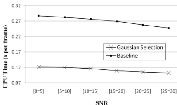
Figure 3: CPU time per frame of 170-Cluster-34-Best Gaussian selection and the baseline recogniser without Gaussian removal on isolated word grammar of SpeechDat Flemish in-car data.
