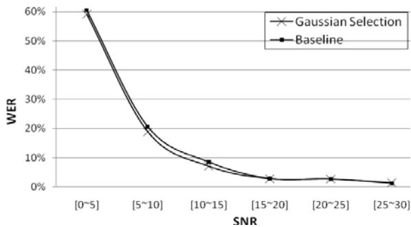
Figure 2: WER per SNR of 170-Cluster-34-Best Gaussian selection and the baseline recogniser without Gaussian removal on isolated words grammar of MIDAS Flemish in-car data
