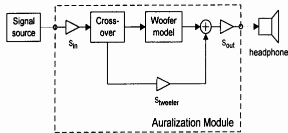
Fig. 6: Auralization of a woofer in multi-channel system
