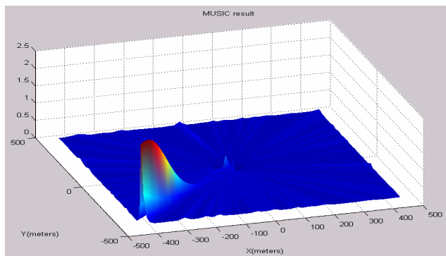
Figure 2: Result of the estimation of the source position with a 17\% \cdot \lambda error on the microphone position knowledge for a 9 microphones array inside a 50x50 m area. Source actual position : -400,-400 ; signal wave length : 3.4 meters
