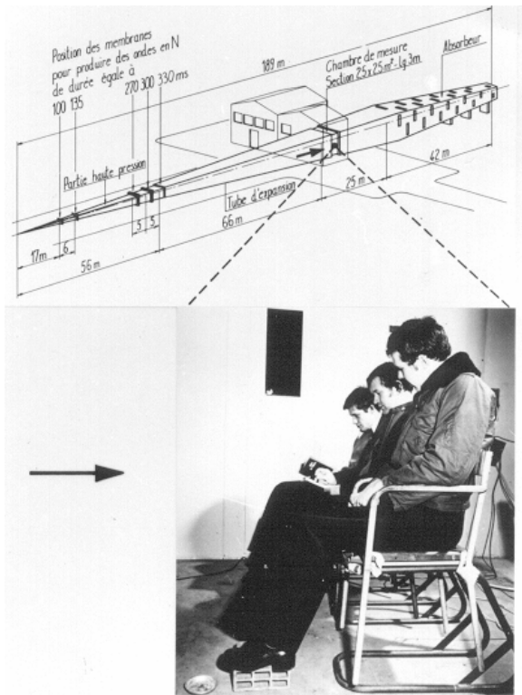
ISL large sonic boom facility
