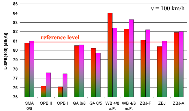
Figure 5: Results of the statistical pass by measurements on ten surfaces in 2002 and 2003.
