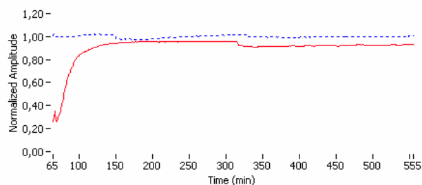
Figure 4: Evolution of the ultrasonic amplitude in the draining grains: grains moulded with air inclusions (average of 4 curves) — grains moulded without air inclusions (average of 4 curves) - - - .
