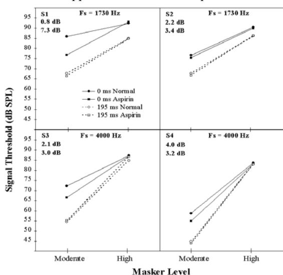
Figure 1: Individual masked thresholds as a function of masker level. The 10-ms signal frequency was 1730 Hz (top row) or 4000 Hz (bottom row). The 400-ms masker was a noise centered at the signal frequency with a width of 10 ERBs.
