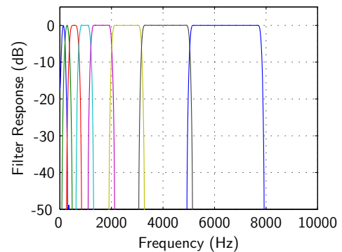
Figure 1: Graphical representation of the 8-channel filterbank response
