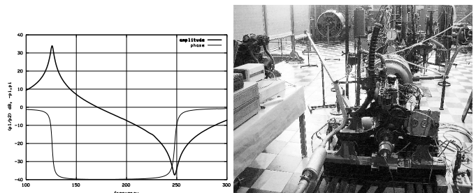
Figure 3: left: Calibration measurement using the closed duct, containing the first pole and first zero of the microphone transfer function. right: Setup to measure the acoustical impedance of a 747 cm 3 combustion engine exhaust.
