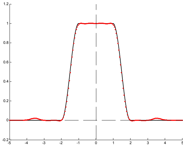
FIG.2 : Reconstruction of a Tukey profile: exponential integration of order 5
