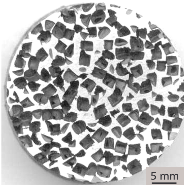
Figure 1: Aluminium-foam sample.
