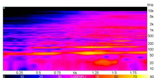
Figure 5 Simulated pass-by (left ear) calculated using near-field component measurement
