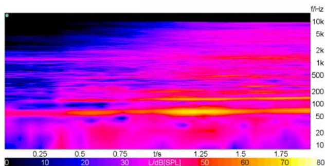
Figure 4 Simulated pass-by (left ear) calculated using far-field array measurement
