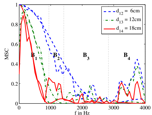
Figure 2: Magnitude squared coherence measured in a car and the theoretically calculated MSCs
