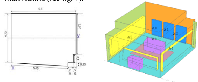
Figure 1: Ground plan of the target room at JOANNEUM RESEARCH (left), room model with absorbers and furniture implemented in CATT Acoustic® (right)
