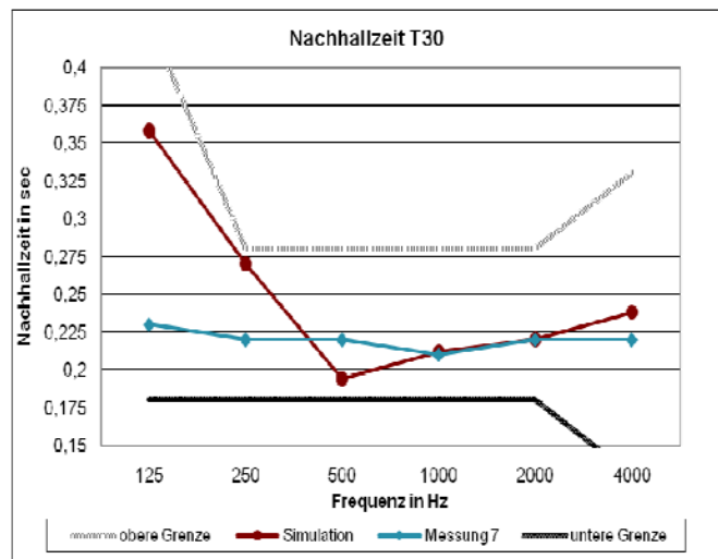
Figure 2: Reverberation time T30 of the equipped listening room (red – simulation, blue – measurement)
