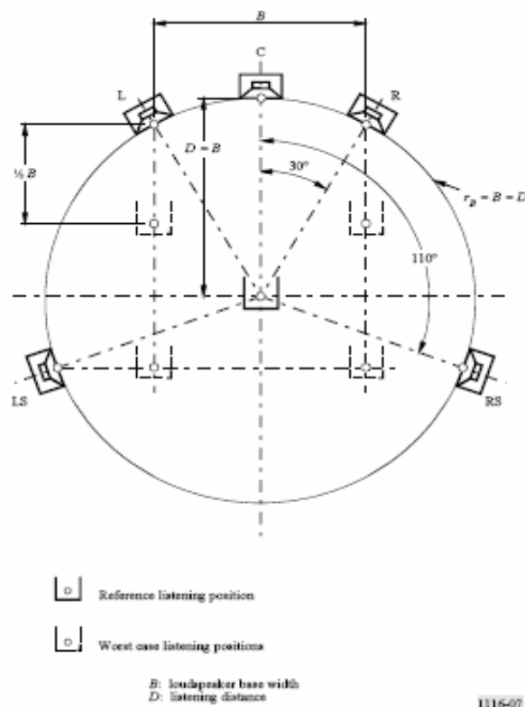
Figure 4: Positioning of the loudspeakers according to the ITU standard’s recommendation
