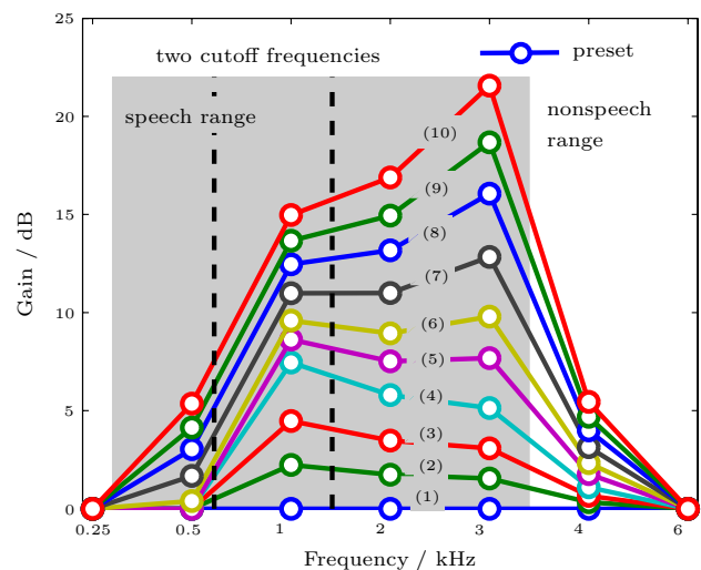
Figure 1: Presets defined by [1], NAL-R and FIG6 at the frequency range of telephone speech signal, i.e. 300 to 3400 Hz; the two cutoff frequencies between the compressor bands are 612 Hz and 1414 Hz.
