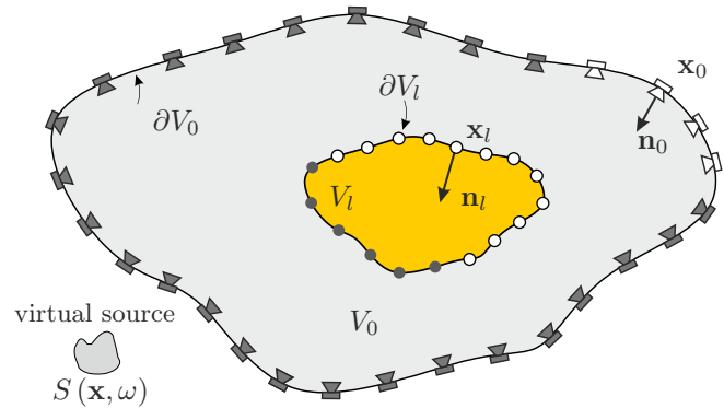
Figure 1: In Local Wave Field Synthesis the desired sound field S(\mathbf{x}, \omega) is reproduced inside the local listening area V_l (yellow shade) with the virtual secondary source distribution (dots) on its boundary \partial V_l . Active virtual secondary sources and loudspeakers are shaded dark.
