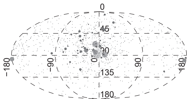
Figure 2: Spatial distribution of the first 100 ms of the employed first-order directional impulse response analyzed by SDM. Brightness and size of the circles indicate the level.
