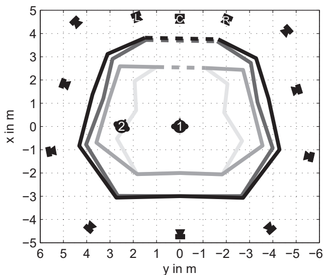
Figure 4: Median sweet spot radius for each loudspeaker direction except C. Gray levels indicate conditions: light gray - 1 st -order original, gray - 1 st -order SDM, dark gray - 3 rd -order SDM, black - 5 th -order SDM.
