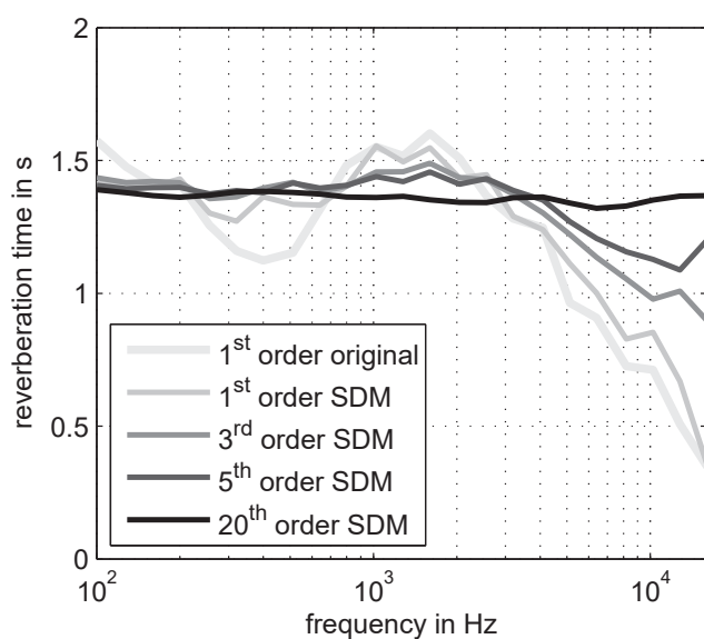
Figure 3: Frequency-dependent reverberation time calculated from original and SDM-enhanced impulse responses.
