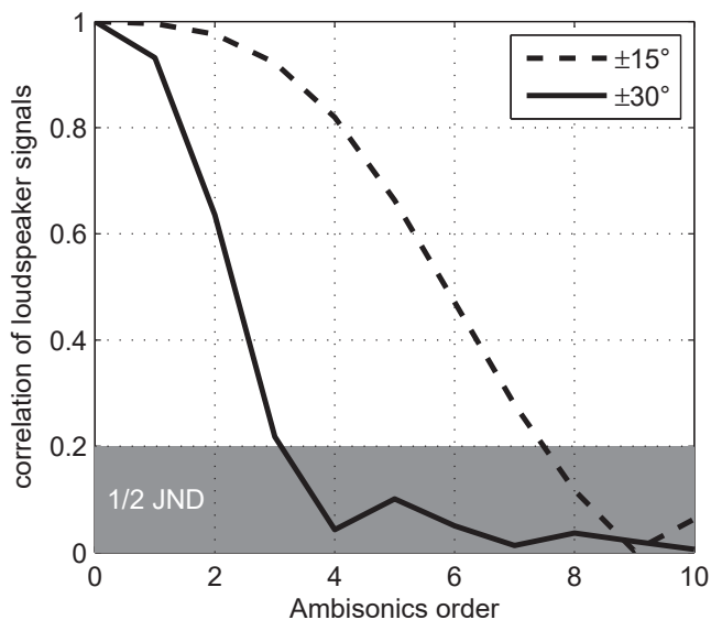
Figure 1: Correlation of 2 independent noise signals at \pm 15^\circ and \pm 30^\circ after Ambisonic encoding/decoding in dependence of Ambisonics order.
