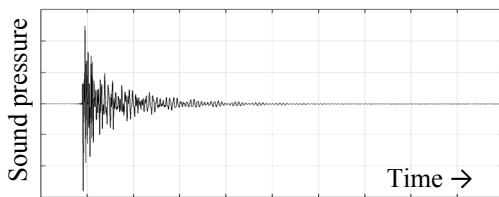
Figure 1: Typical transient signal for FETT. After a sharp increase in sound pressure, a damped decay follows.
