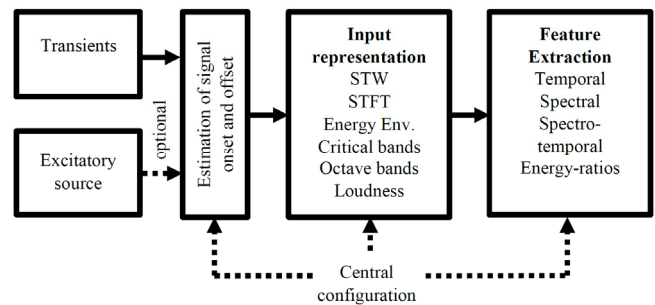
Figure 2: Stepwise process from input to features as done by FETT. Input from excitatory source (e.g. impulse hammer) is optional. A central configuration table store all necessary parameters for estimation of signal boundaries (onset and end), input representation and feature extraction.
