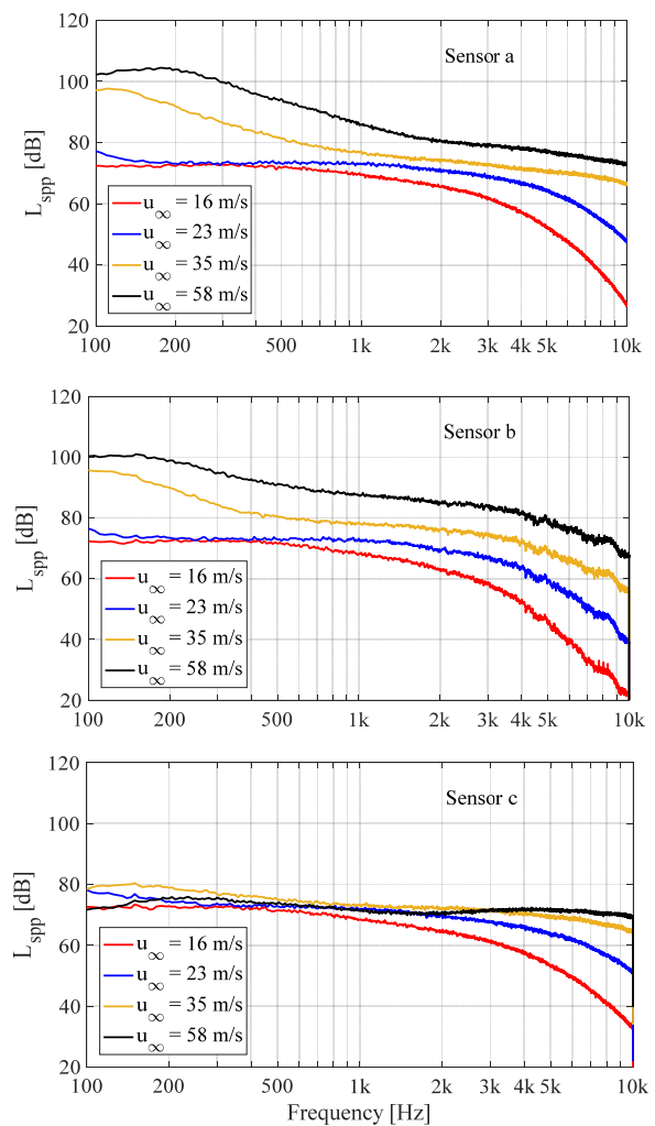
Fig. 4 PSDL of hydrodynamic pressure fluctuations obtained with sensor a, b and c; sensor c is not suitable for the level of the test signals applied.
