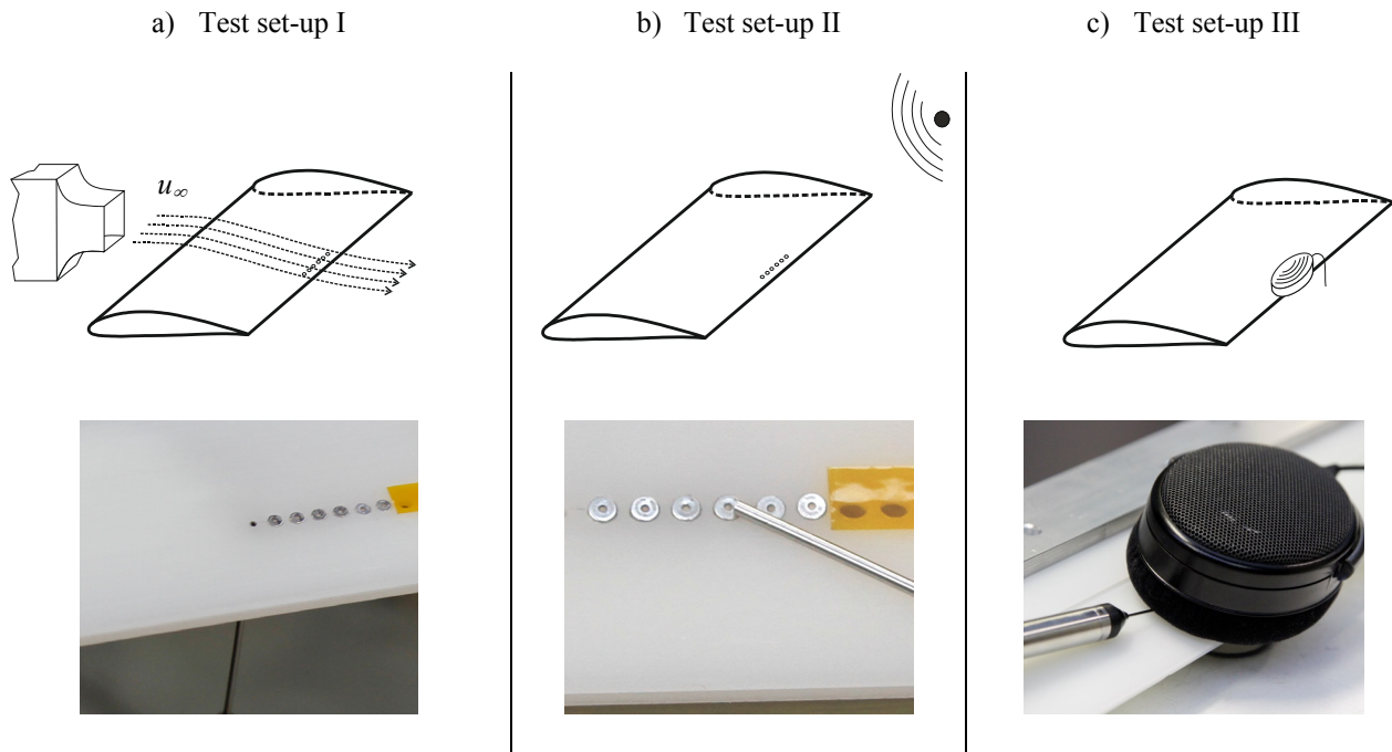
Fig. 3 Test set ups: a) hydrodynamic b) acoustic signal from free field sound source, c) acoustic signal from headphone
