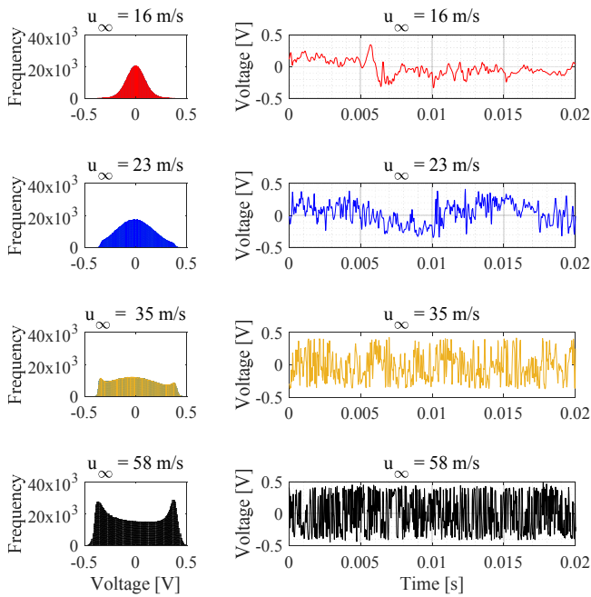
Fig. 5 Time traces and amplitude histograms of the raw signal from sensor c for increasing flow velocity; clipping is clearly visible for u_\infty \geq 35 m/s.
