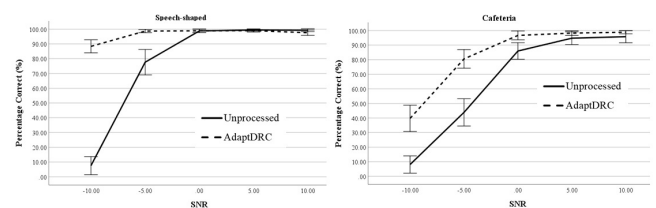
Figure 1: Mean words correct in percent. Error bars show 95% confidence intervals.
