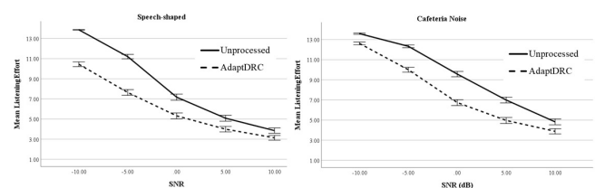
Figure 2: Mean listening effort ratings in Effort Scaling Categorical Units. Error bars show 95% confidence intervals
